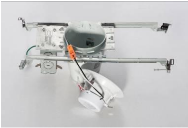
Step2: Insert male connector into female one.
